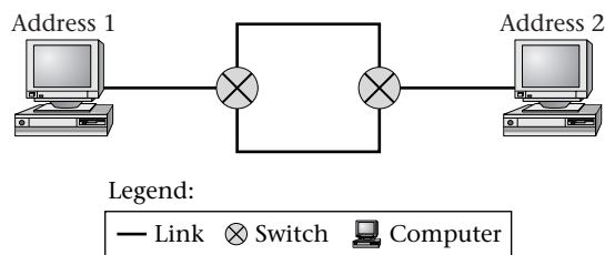
Figure 9.1 This network (or internet) contains four links, two switches, and two interfaced computers. Two alternative paths connect the two computers. As described in the text, more information would be needed to determine whether this is a picture of a single network or an interconnected group of networks, that is, an internet.
