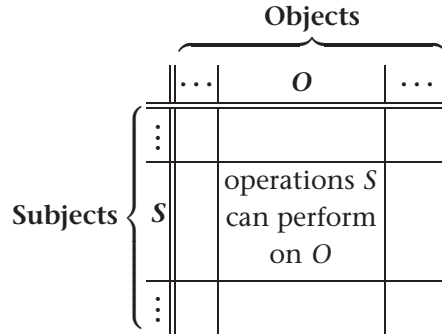
Figure 7.10 An access matrix has one row for each subject, one column for each object, and entries showing which operations each subject can perform on each object.
